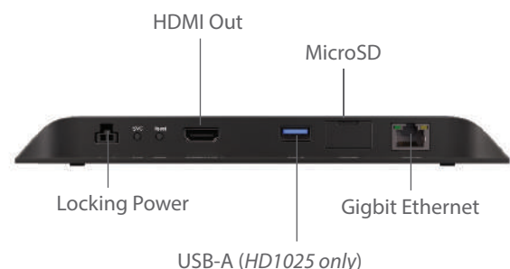
Back View
